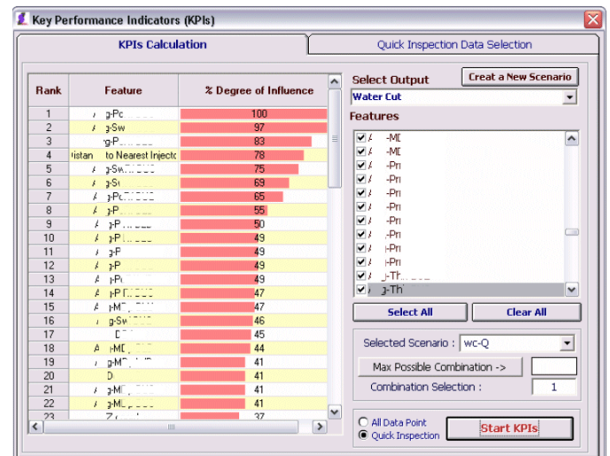
Figure 6. Key Performance Indicators identified for the SRM development.
