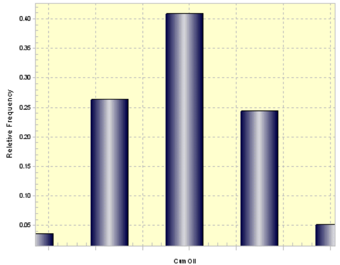
Figure 14. Probability distribution function for cumulative oil.
