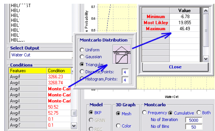
Figure 10. Assigning pdf to specific parameters in SRM.
