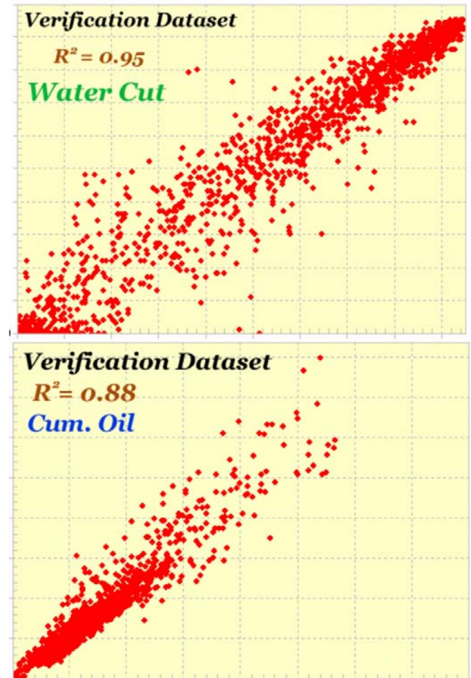
Figure 8. Validation of the Surrogate Reservoir Model using 40% of the data that was not used during its development. Here actual FFM outputs are plotted against SRM's predictions.
